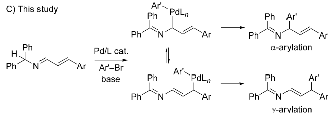
Scheme 1. Arylation of azaallyl anions.
